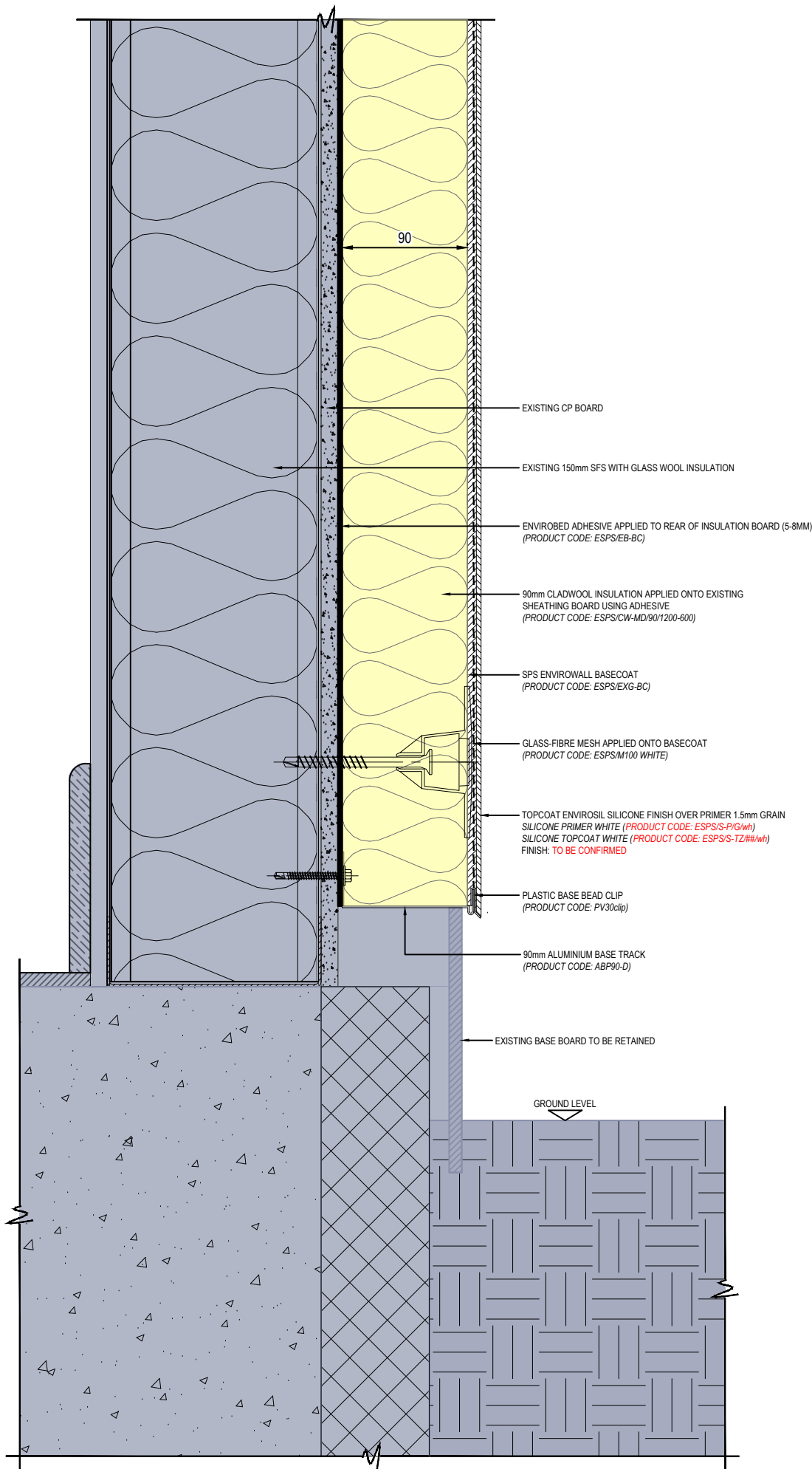
01 PLAN SECTION - RENDER / BOARD TO RAISED BEDS Scale 1:2
